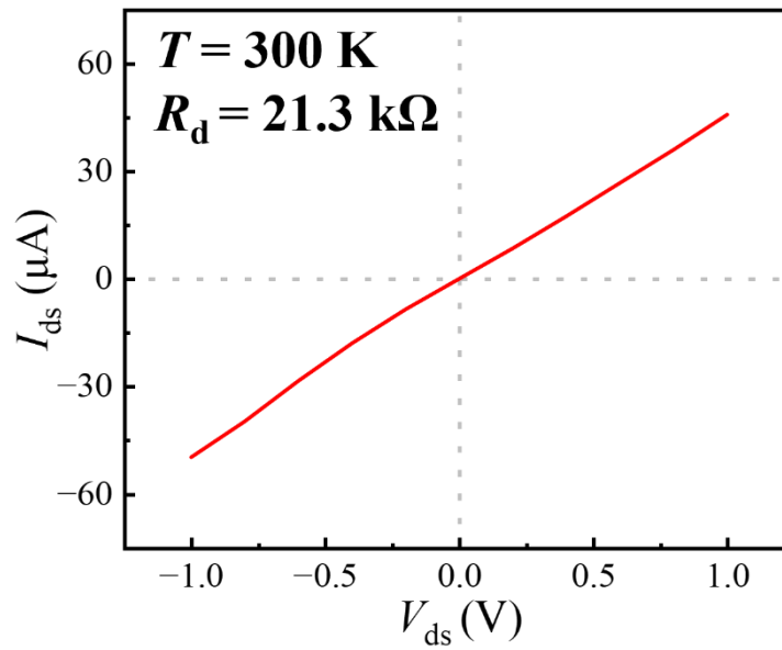
Fig. S1. Output curve of b-As 0.5 P 0.5 device.
